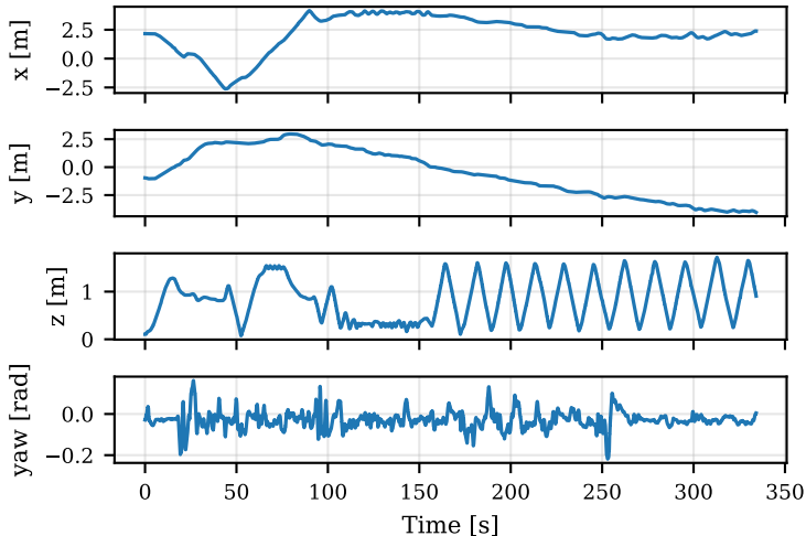
exp 1 - UAV 2 - Position
